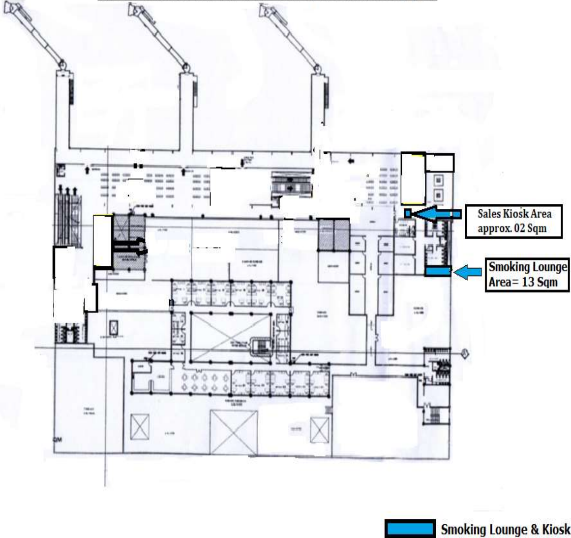
Floor Plan for SHA (First Floor) at Jammu Airport
