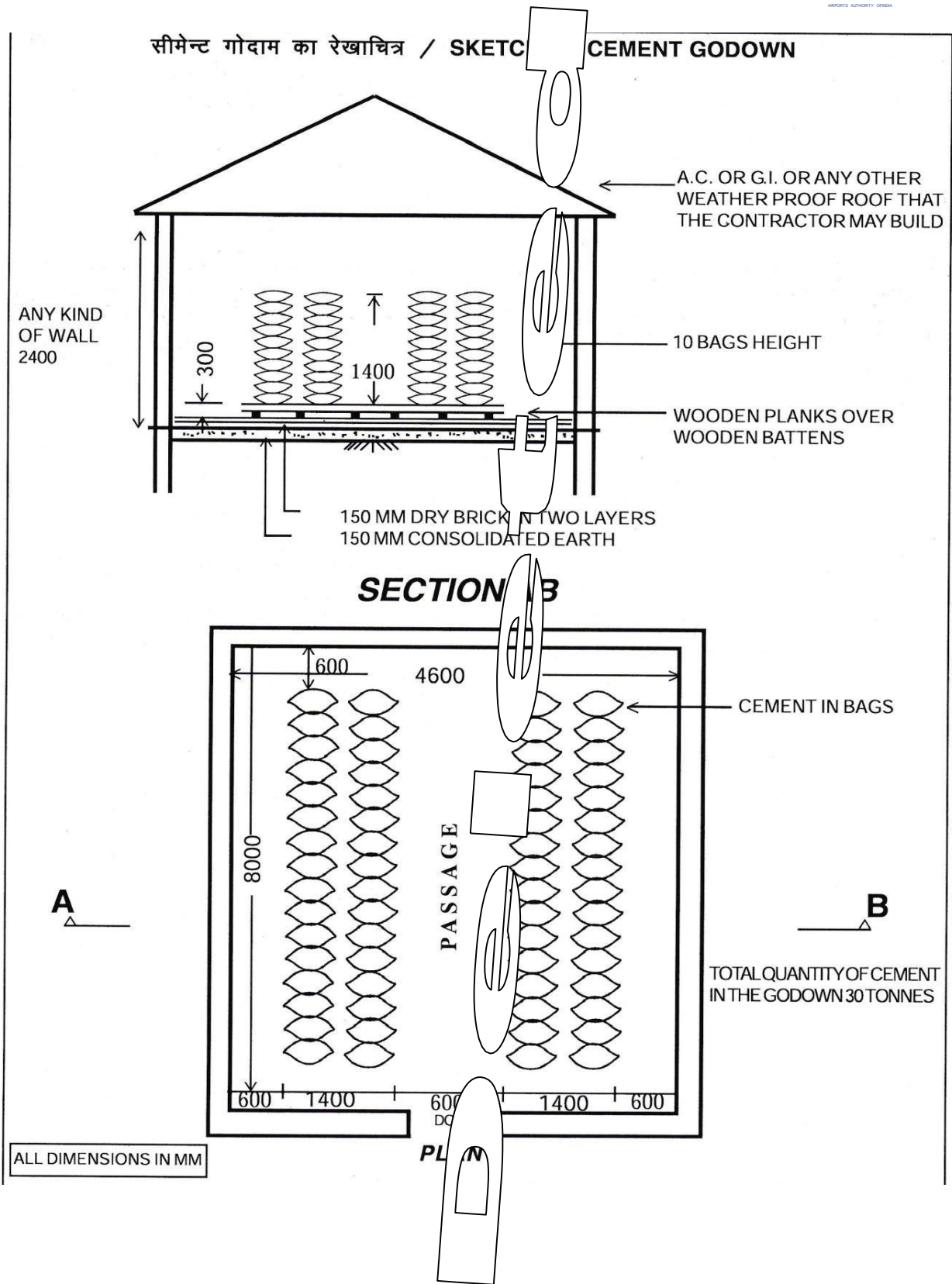
SKETCH OF CEMENT GODOWN
