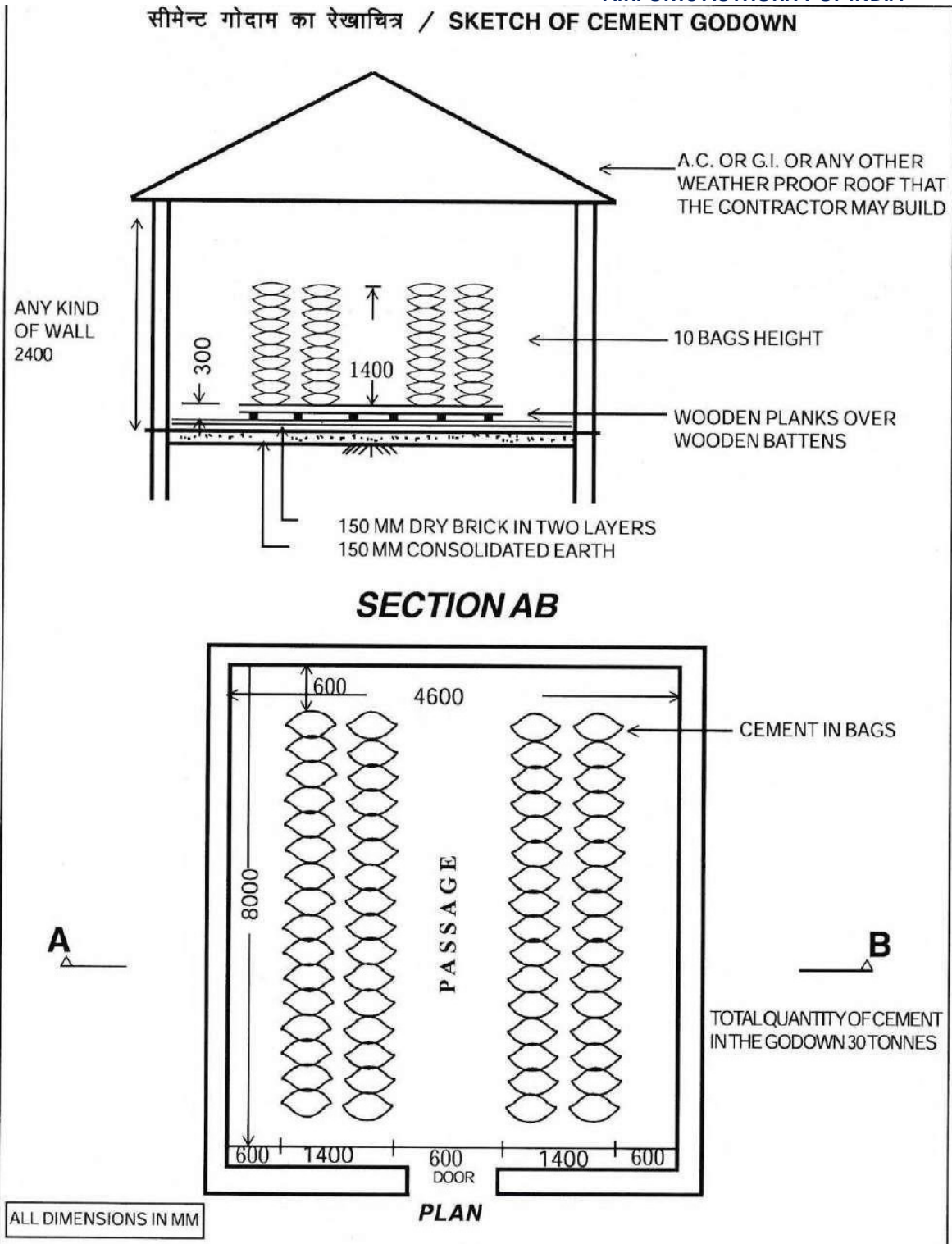
SKETCH OF CEMENT GODOWN
