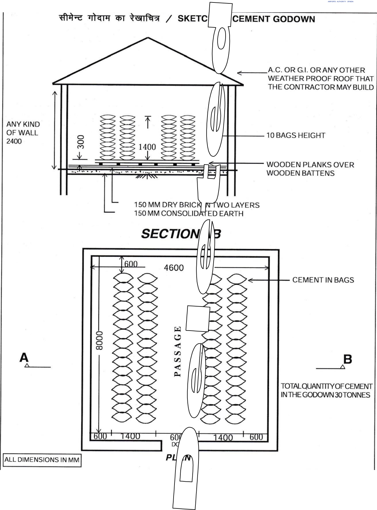
SKETCH OF CEMENT GODOWN
