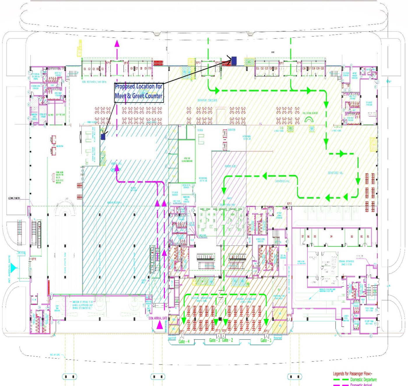
Ground Floor Commercial Layout Plan of Vadodra Airport
